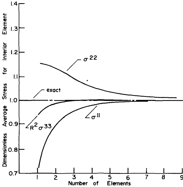
FIG. 9. Convergence of average stress-interior element.
